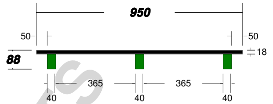
End View
